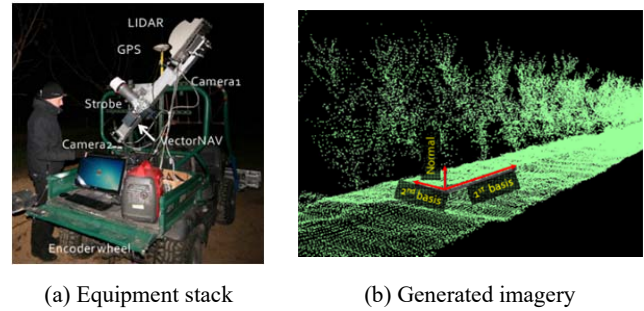
(a) Equipment stack (b) Generated imagery Fig. 16 LIDAR system for orchard mapping, sensor and feature extraction [54]
